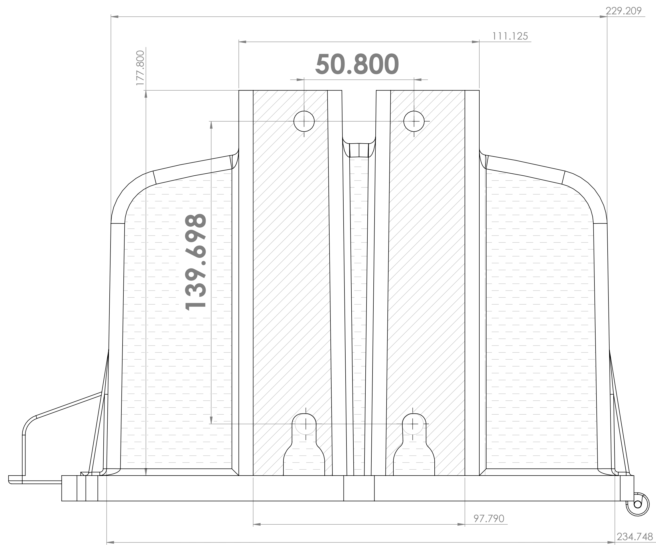
3/8" Dia. Bolt Clearance Holes/ Key slots (4)
